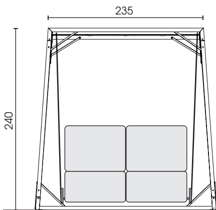
Front side, rocking frame
