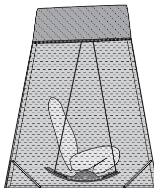
Side view, rocking frame with sun canopy and weather protection
