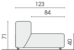
Side view, height with 5 cm feet
